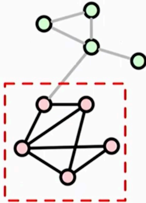
Quasi-complete
